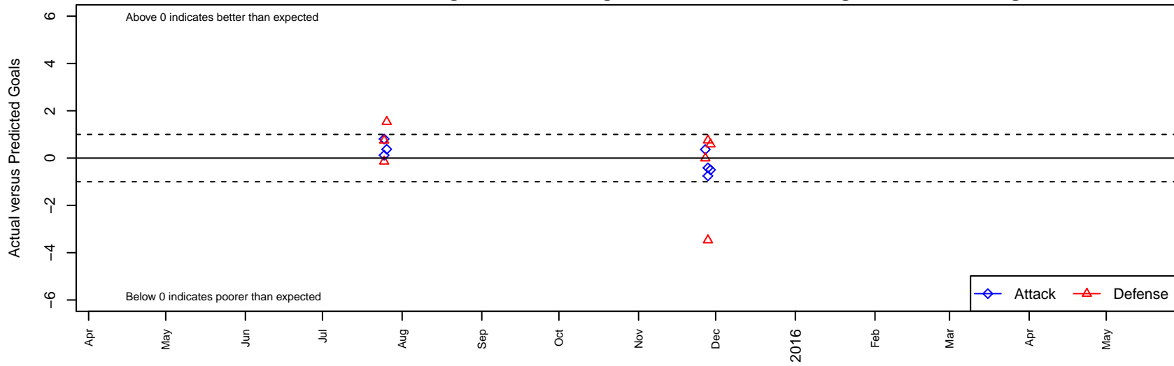
Santa Rosa United Tremors G99 Dots are actual minus expected GF (blue circles) and GA (red triangles). Blue line is smoothed change in attack strength. Red is smoothed change in defense strength.
